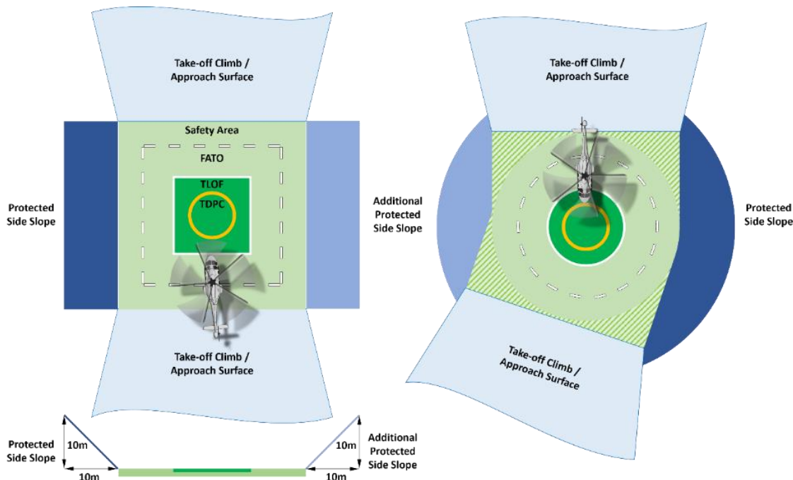
Figure 7: Basic features of onshore heliports
