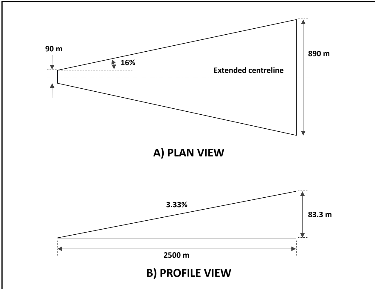
Figure 16: Approach surface for non-precision approach FATOs
