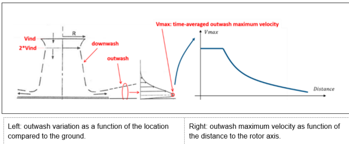
Figure 6: Demonstration of rotor downwash, outwash and maximum velocities
