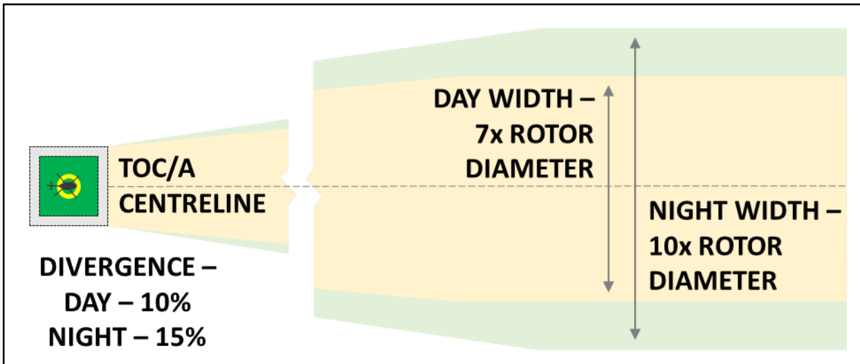
Figure 13: Overview of take-off climb/approach surface for non-instrument FATOs
