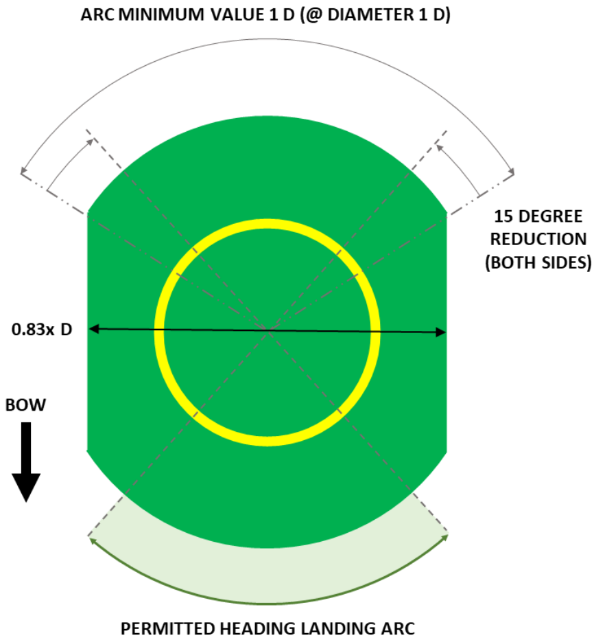
Figure 12: Shipboard permitted landing headings for limited heading operations
