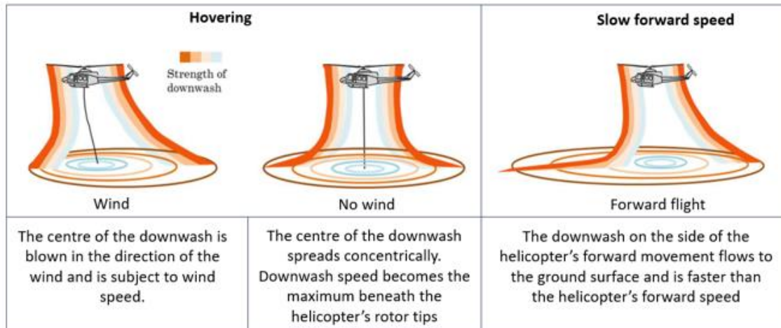
Figure 4: The impact of wind on helicopter downwash
