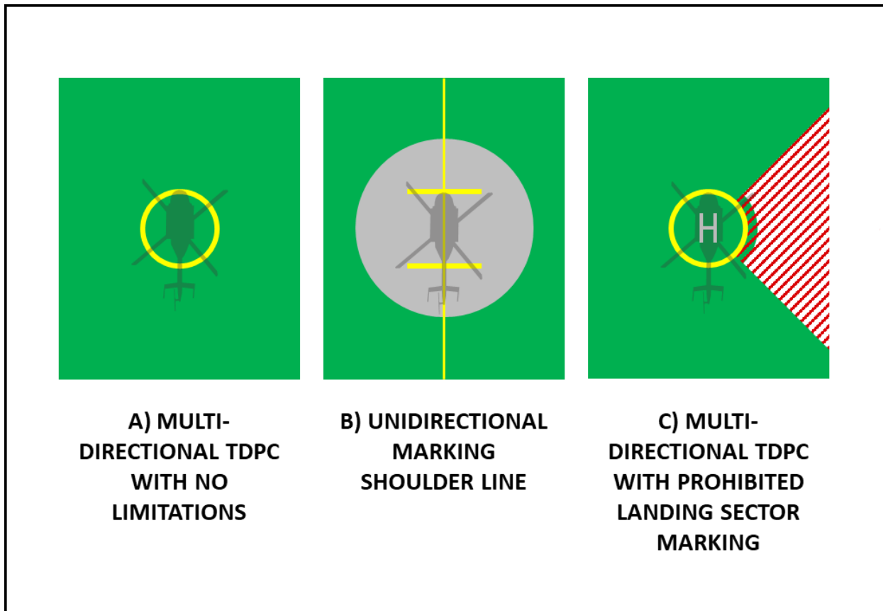
Figure 28: Examples of touchdown/positioning markings
