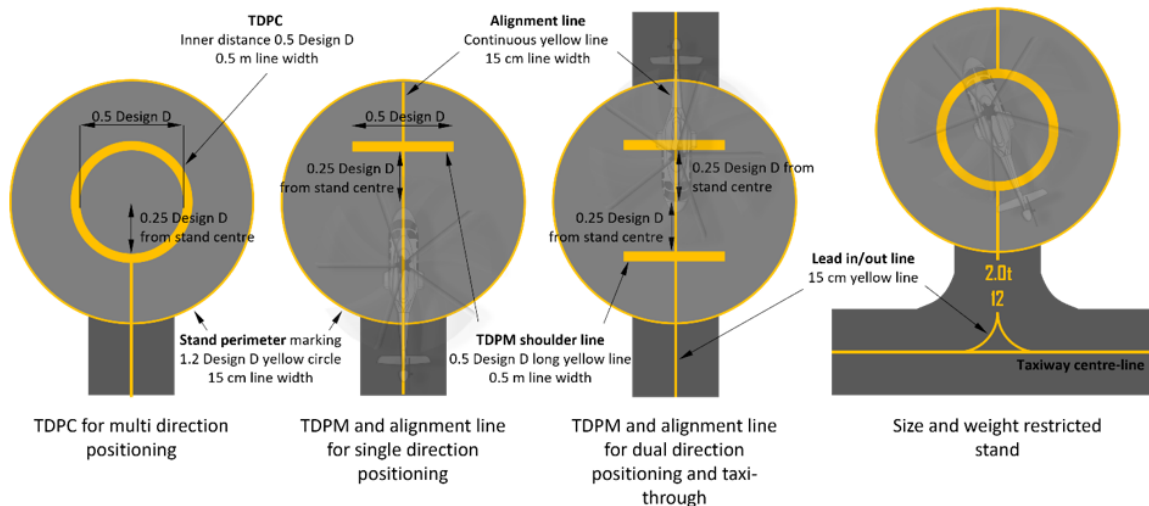
Figure 29: Helicopter stand markings
