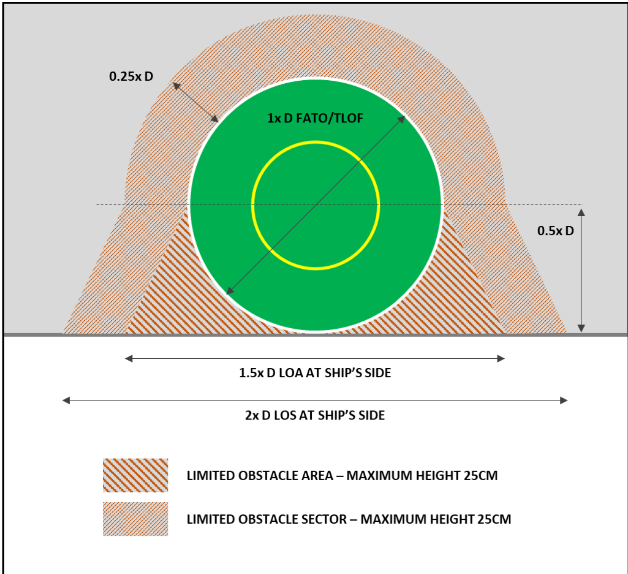
Figure 22: Ships-side non-purpose-built shipboard heliport obstacle limitation sectors and surfaces
