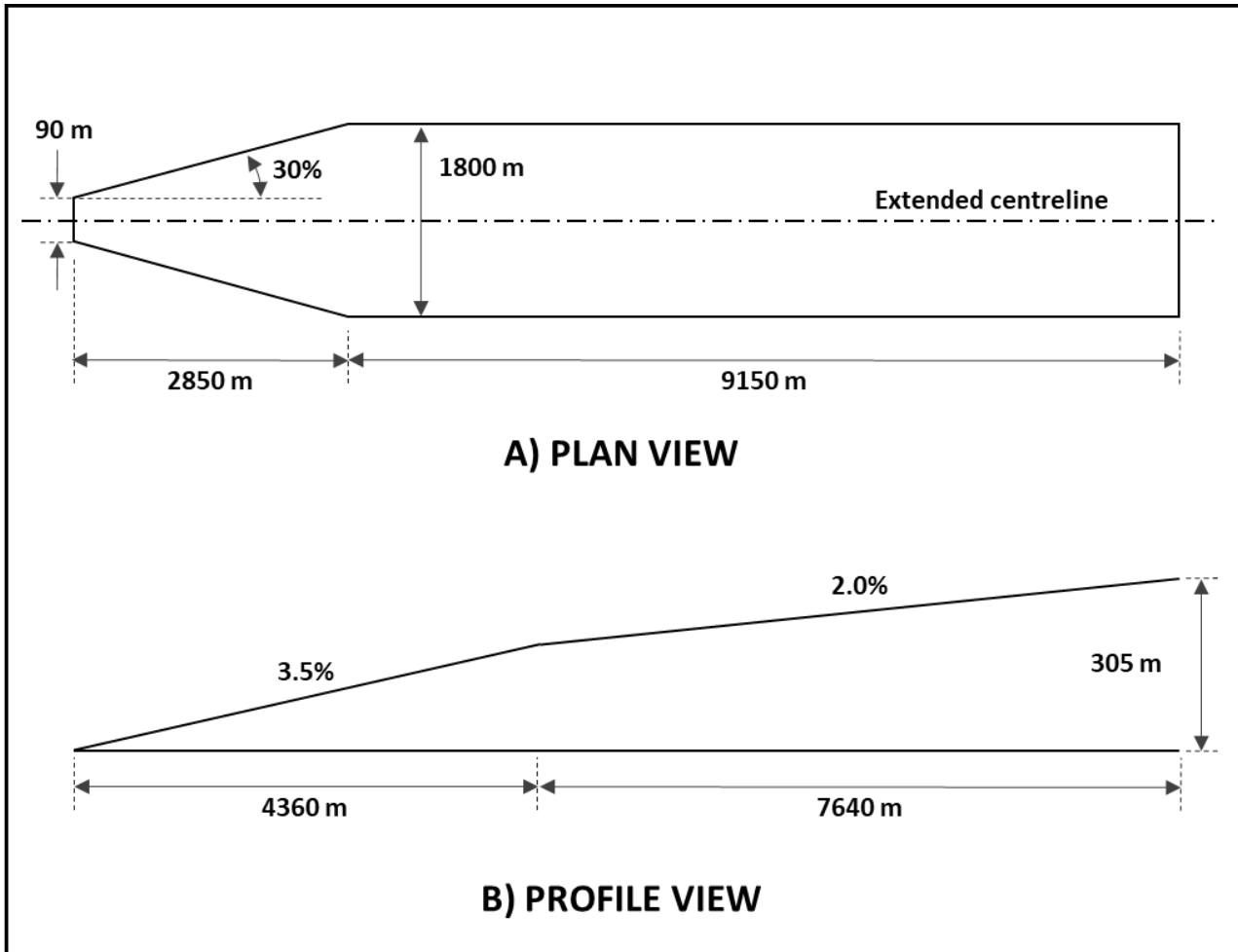
Figure 18: Take-off climb surface for instrument FATOs with straight take-offs
