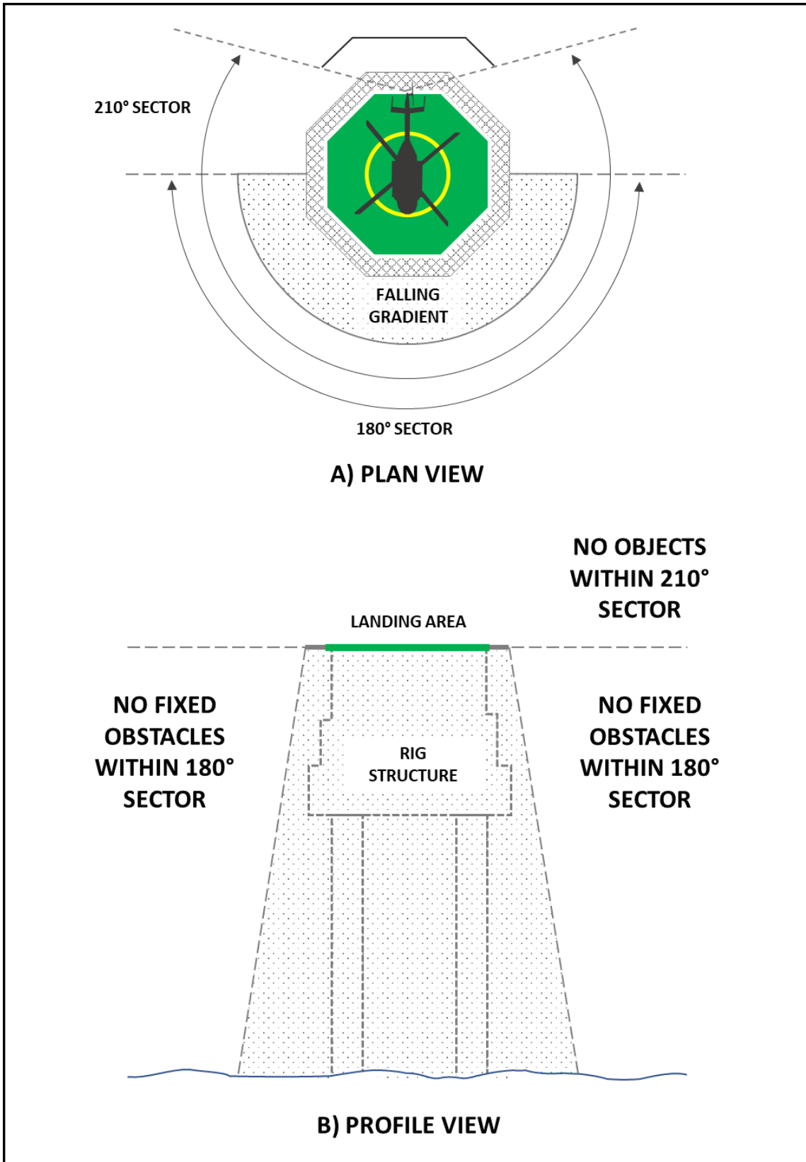
Figure 19: Helideck obstacle-free sector overview
