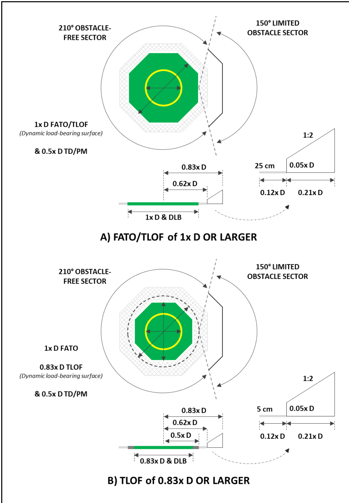
Figure 20: Helideck obstacle limitation surfaces and sectors
