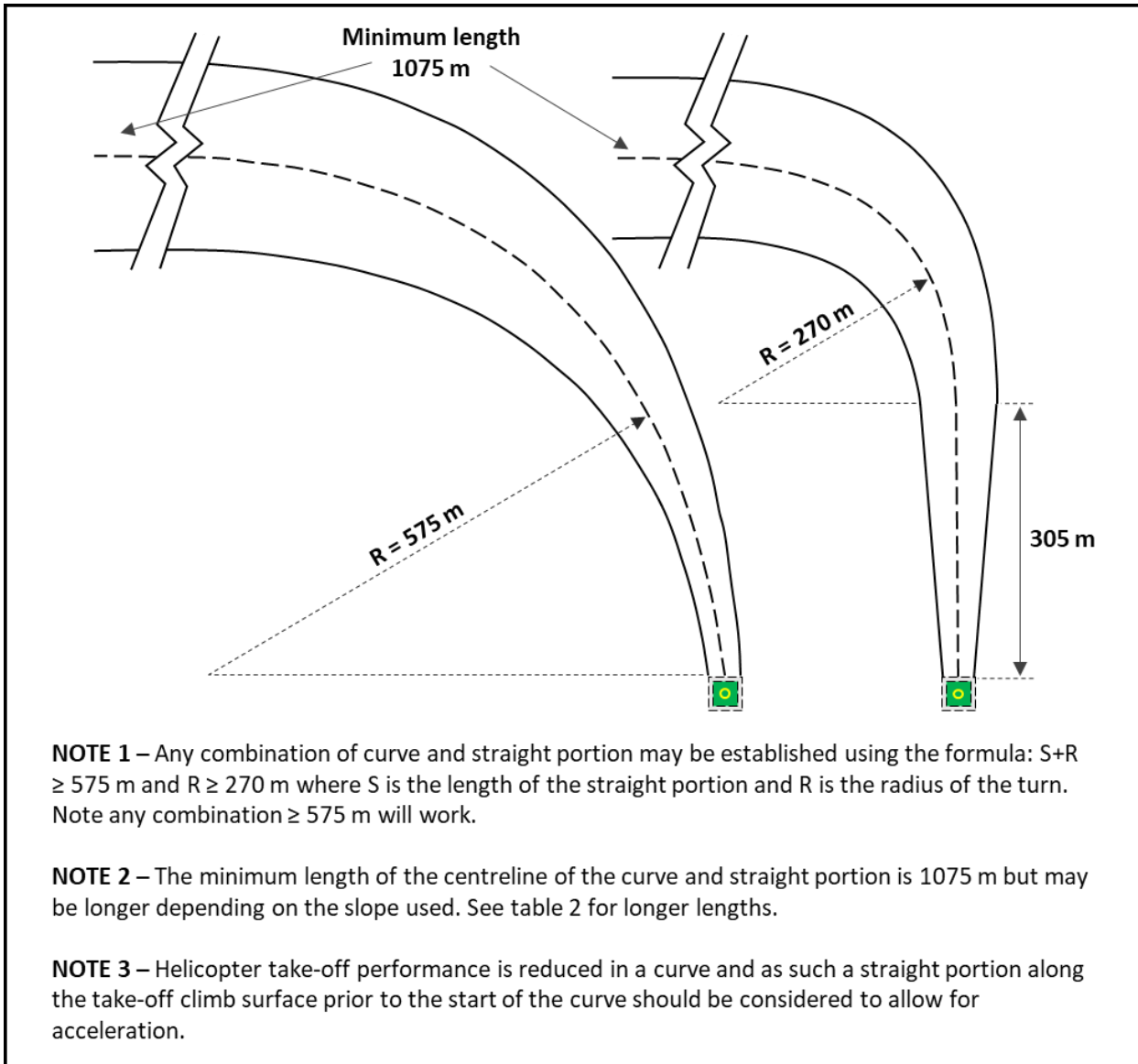
Figure 14: Curved approach & take-off climb surface for all FATOs
