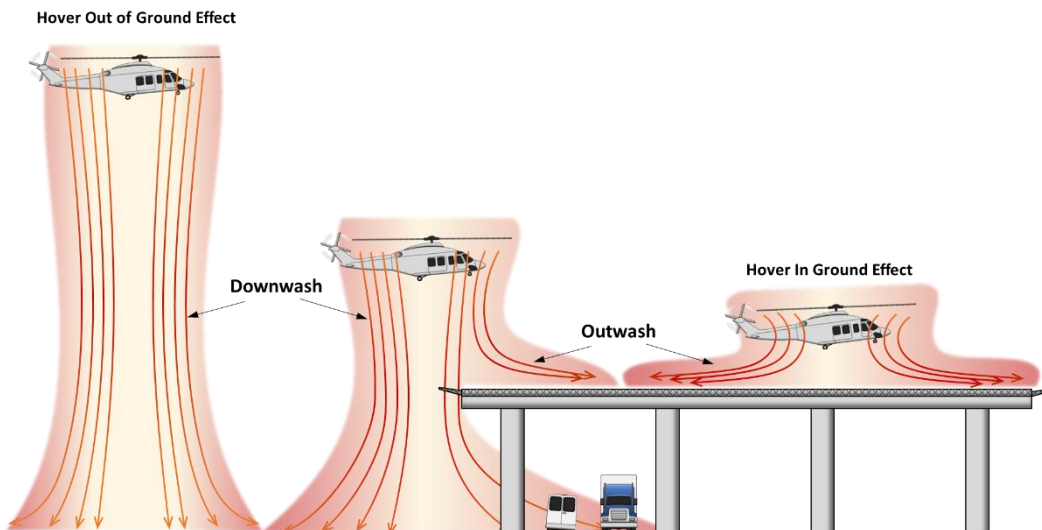
Figure 3: Generalised depiction of down wash and outwash
