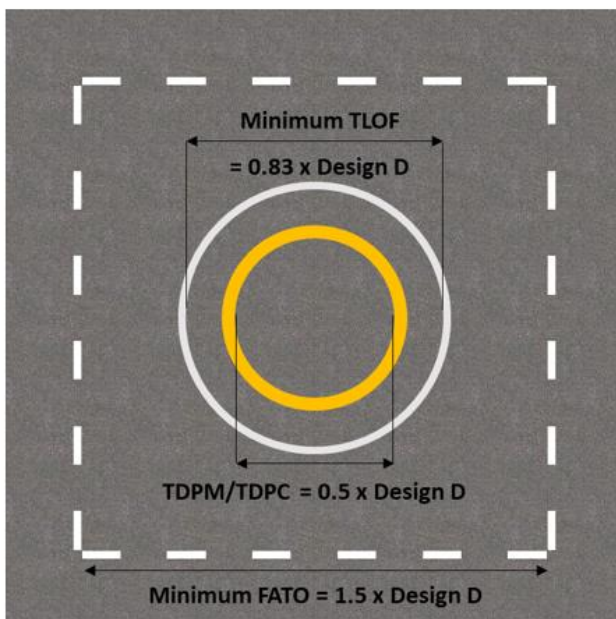
Figure 8: FATO and TLOF dimensions
