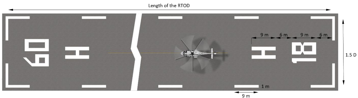
Figure 26: Runway type FATO marking example
