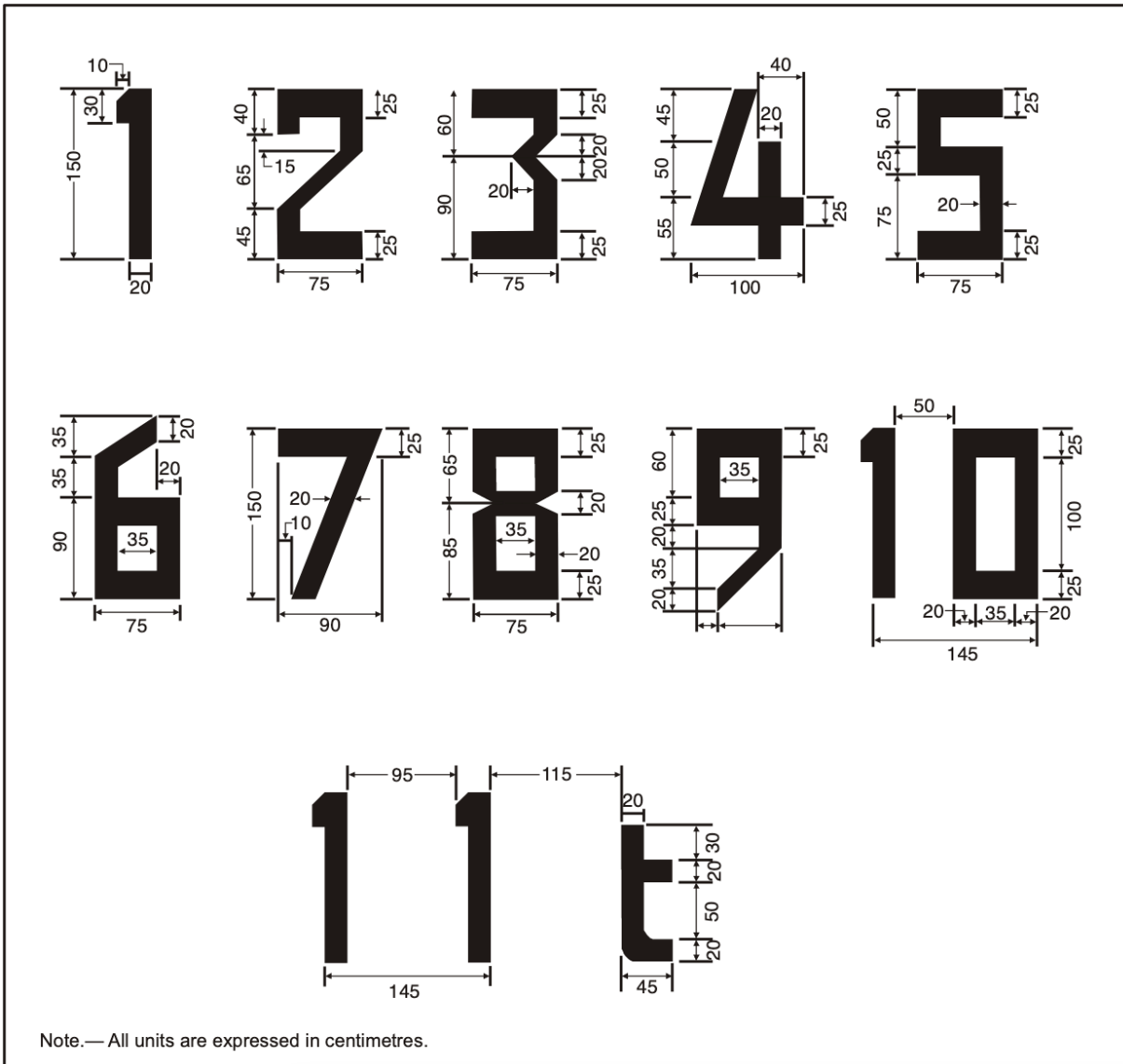
Figure 27: Form and proportion of numbers and letters
