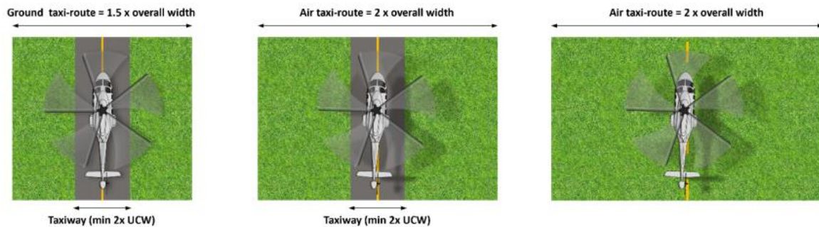
Figure 9: Taxi route examples
