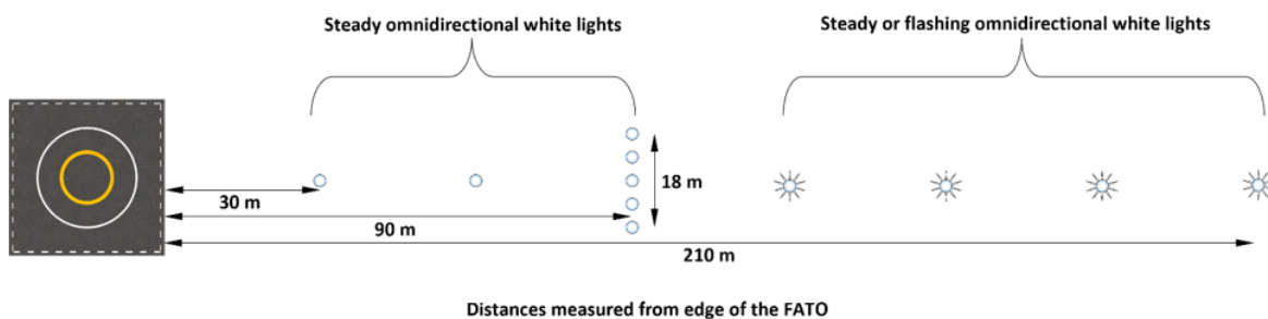
Figure 31: Approach lighting system
