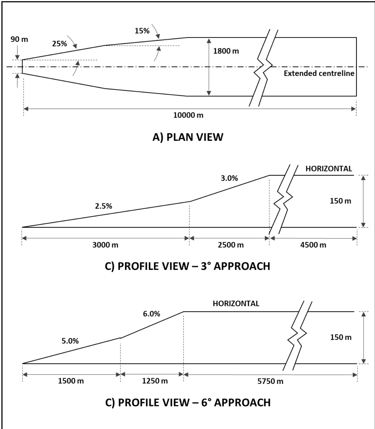
Figure 17: Approach surface for precision approach FATOs
