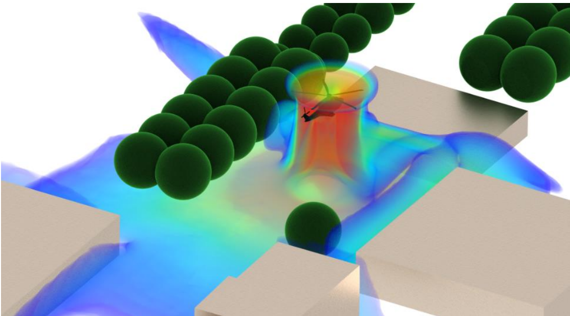
Figure 5: Computer generated fluid dynamics illustration of complex downwash and outwash interactions with structures. Image courtesy of Synergetics (2023)
