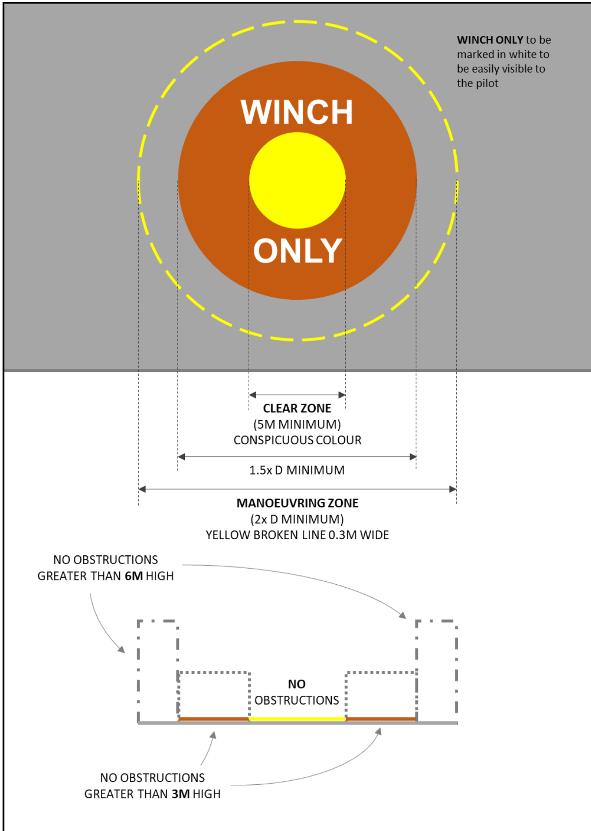
Figure 23: Shipboard winching area obstacle limitations and markings
