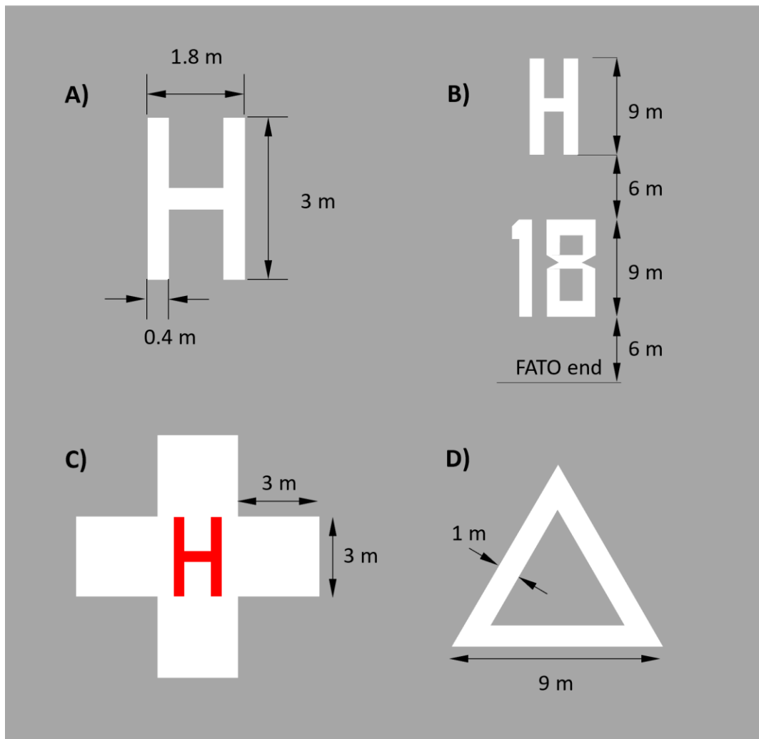
Figure 24: a) Helicopter identification marking. b) Runway type FATO identification markings. c) Hospital heliport identification marking. d) Aiming point marking.
