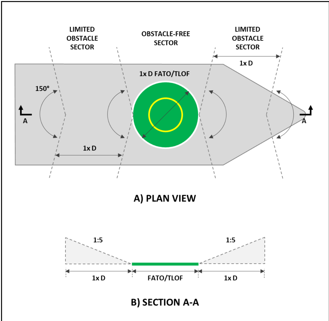
Figure 21: Amidships location – shipboard heliport obstacle limitation surfaces
