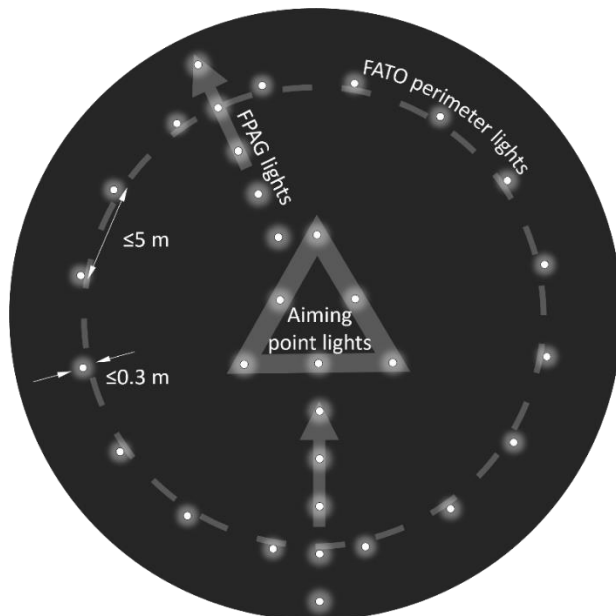
Figure 32: FPAG lights, FATO perimeter and aiming point lights
