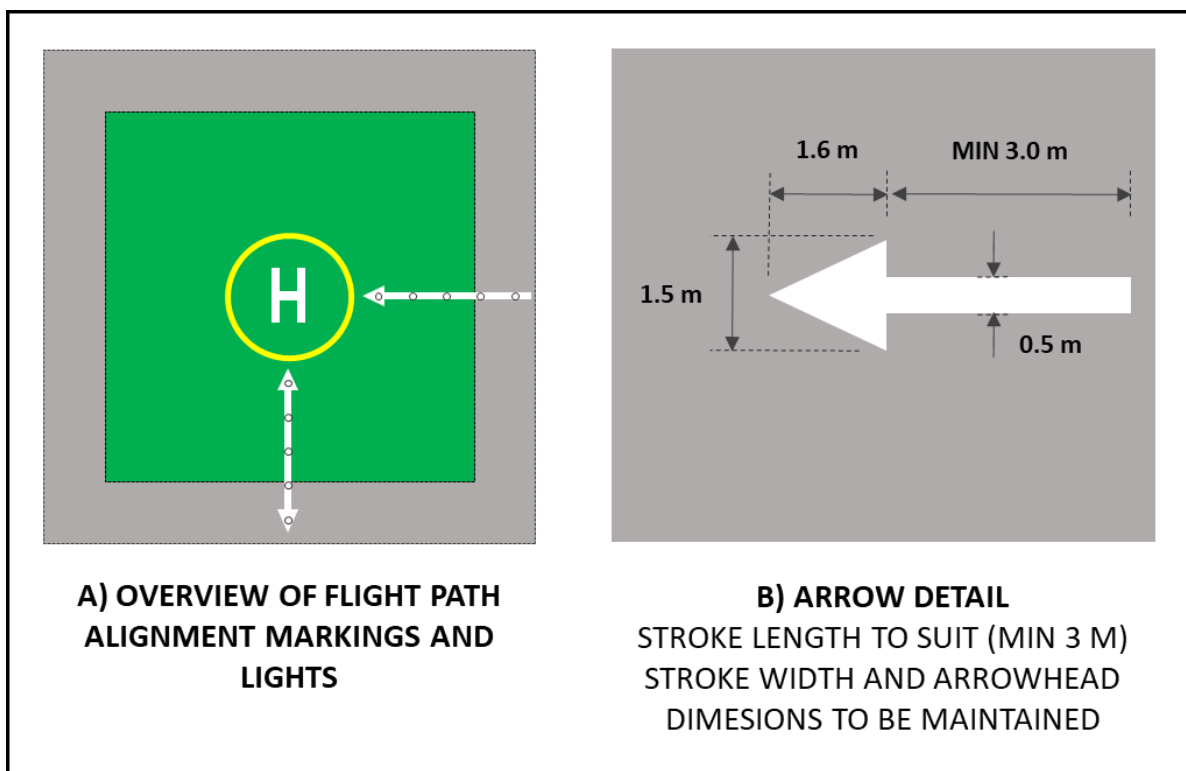
Figure 30: Flight path alignment guidance markings and lights
