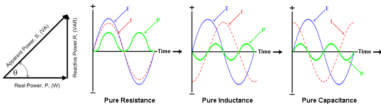
Figure 6: Power triangle and phase relationship
