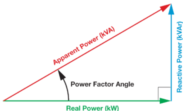
Figure 2: AC power triangle
